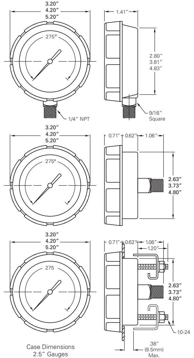
Stud Location 2.5" Case 2:00 and 8:00 Positions 3.5" & 4.5" Case 3:00 and 9:00 Positions
