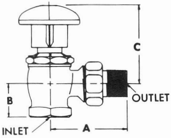
FIG. 1 MODEL AP1
