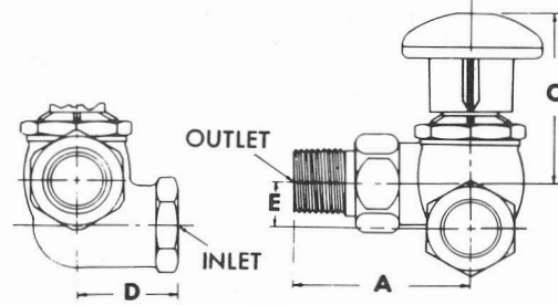
FIG. 8 MODEL LH1
