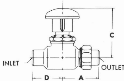
FIG. 5 MODEL ST2
